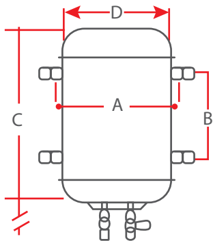
Vertical Mounting
